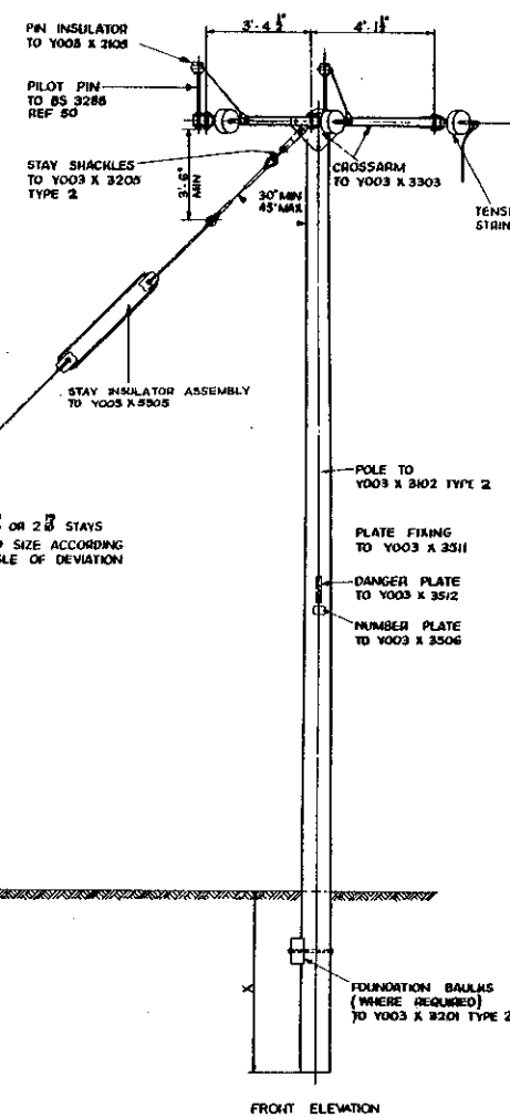
FRONT ELEVATION
